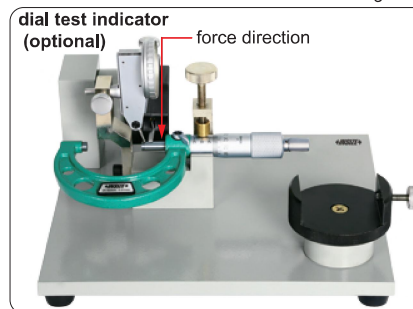
measuring radial swing of spindle
