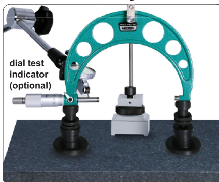
measuring relative offset between the two measuring surfaces
