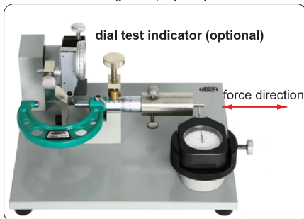
measuring axial play of spindle
