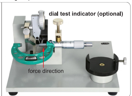
measuring radial swing of spindle
